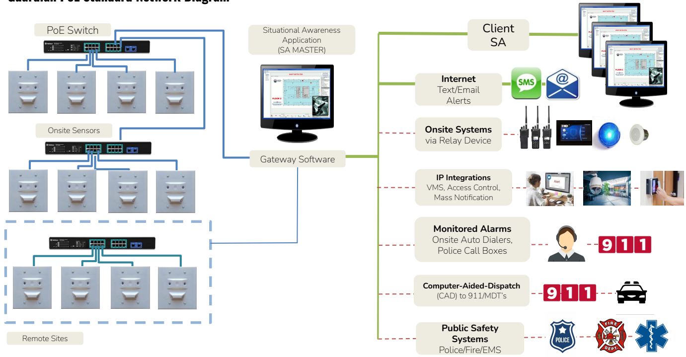
Guardian PoE Standard Network Diagram
